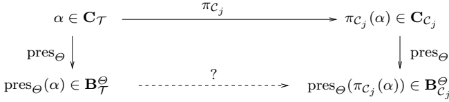
Fig. 1. Extracting behaviour from team automata to component automata.
