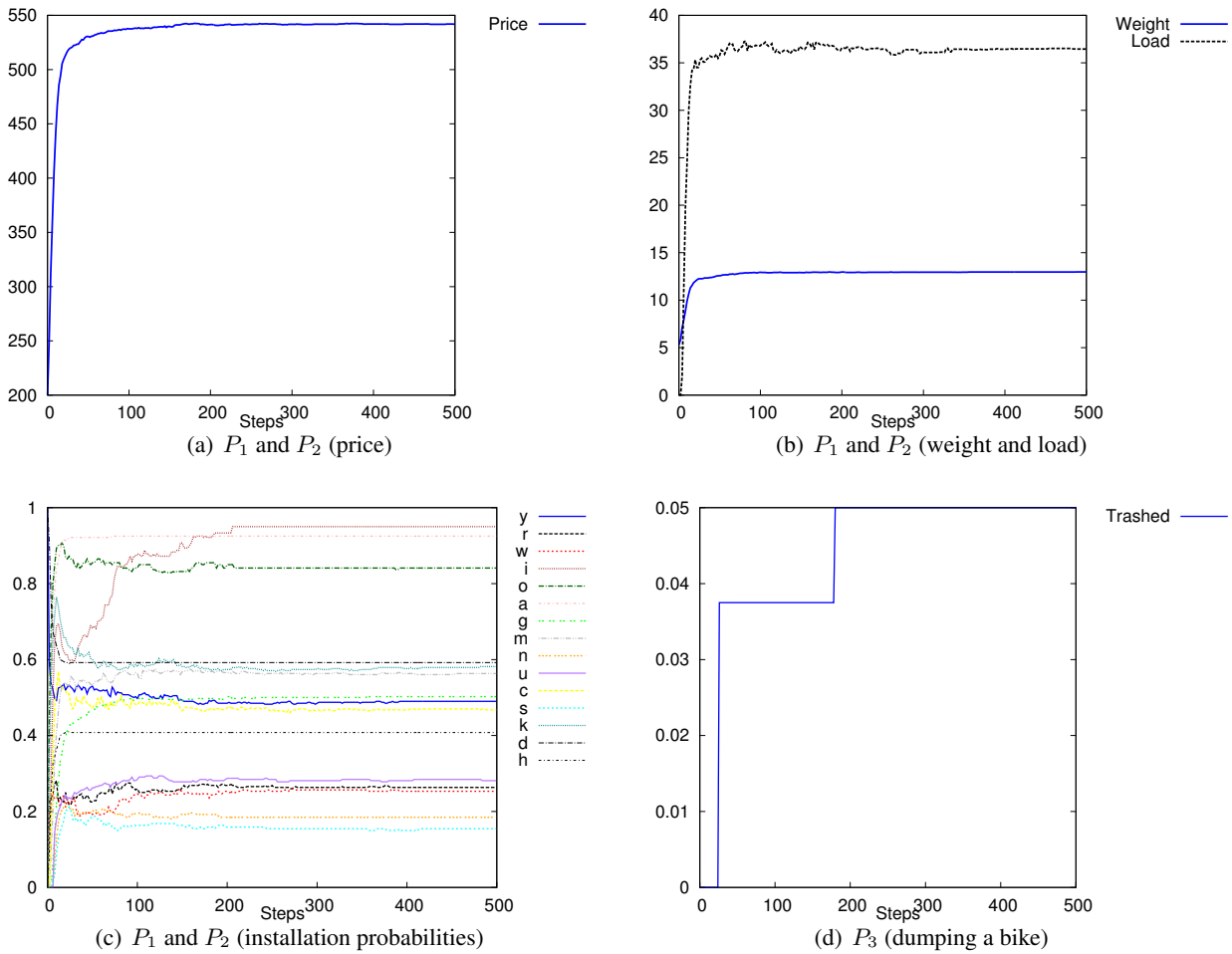
Figure 6: Results of measuring P_1 – P_3 with MultiVeStA
