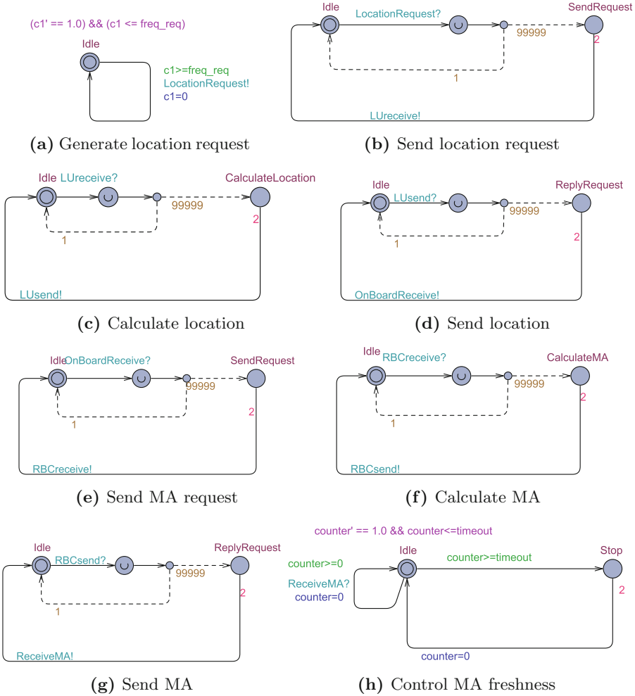
Fig. 2. Complete UPPAAL model of moving block signalling scenario (Color figure online)
